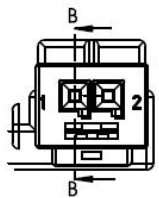
VERSION I / Variante I (WITHOUT LOCKING PART / ohne Anreihelment)
