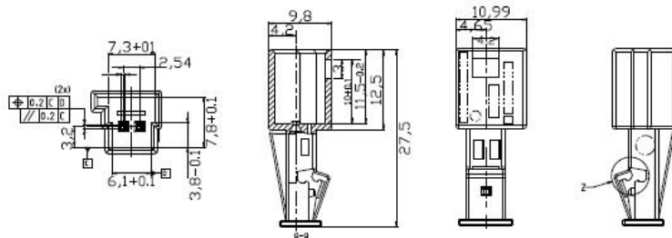
VERSION I / Variante I (WITHOUT LOCKING PART / ohne Anreihelment)
