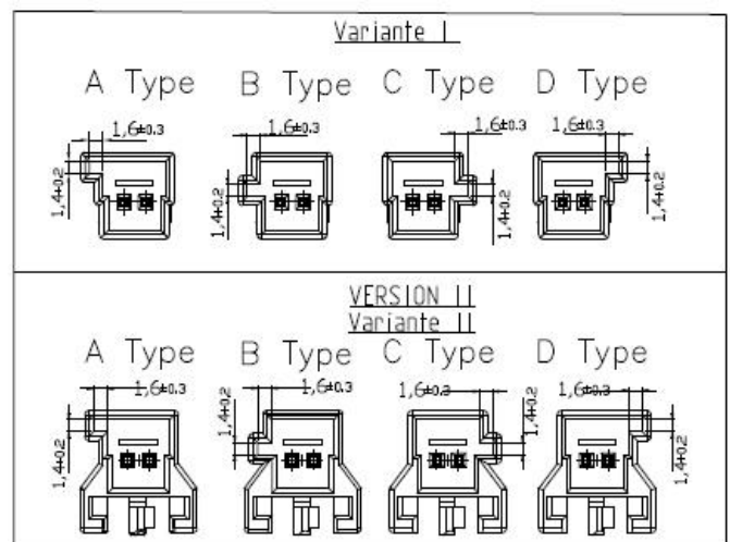
VERSION I / Variante I (WITHOUT LOCKING PART / ohne Anreihelment)
