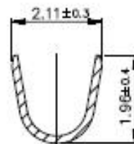
SECTION W—W
