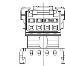
VIEW OF 4 CIRCUIT
