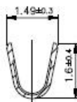
SECTION Z—Z
