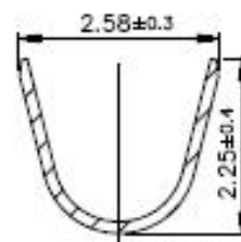
SECTION Y—Y
