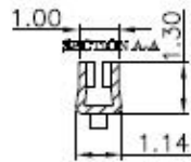
SECTION C-C
