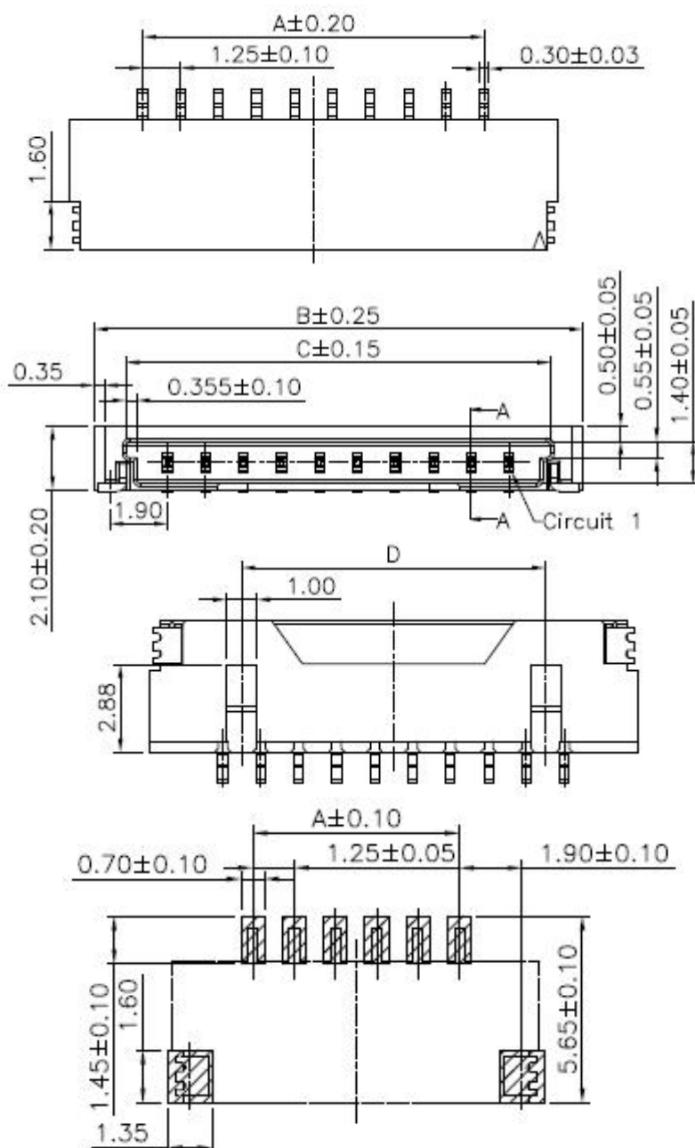
PCB LAYOUT(TOP VIEW)
