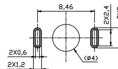
PCB LAYOUT (TOP VIEW) Tolerance: ±0.05mm
