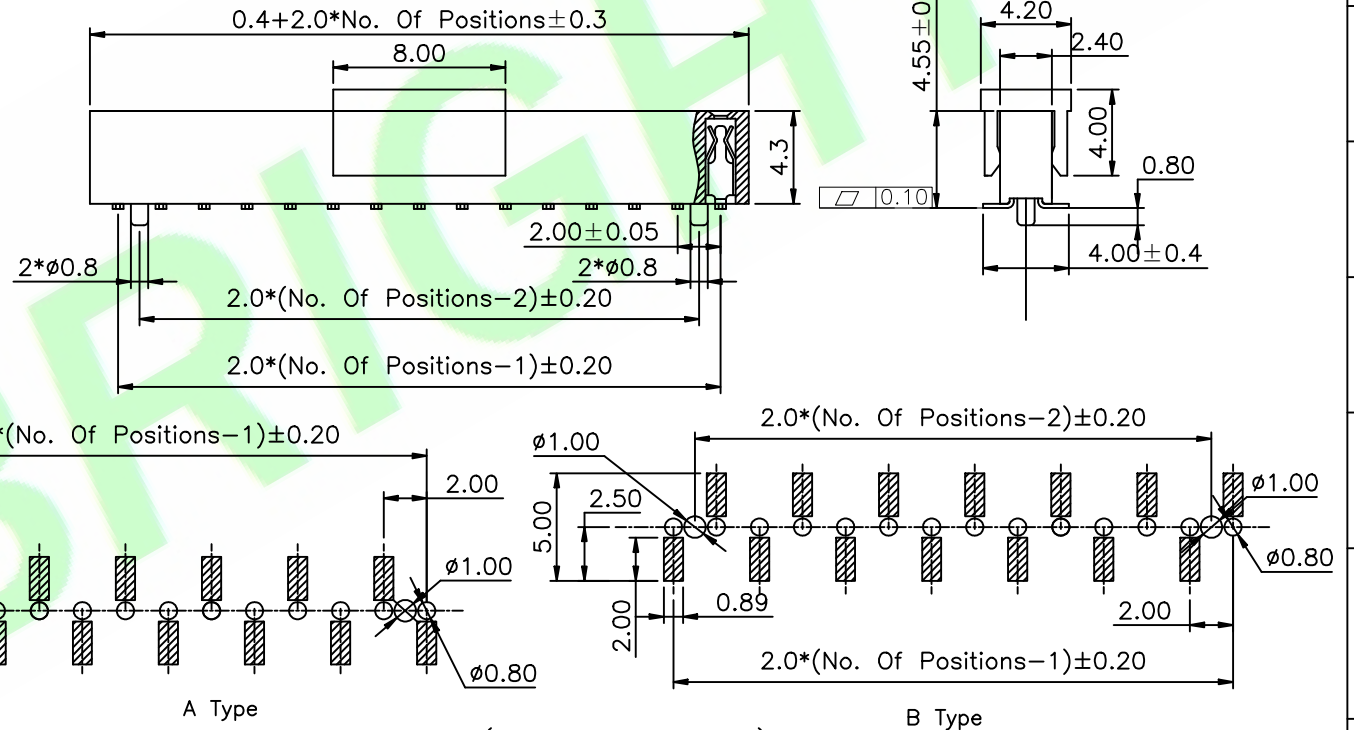
Recommended PCB Layout(Tolerance:0.05mm)
