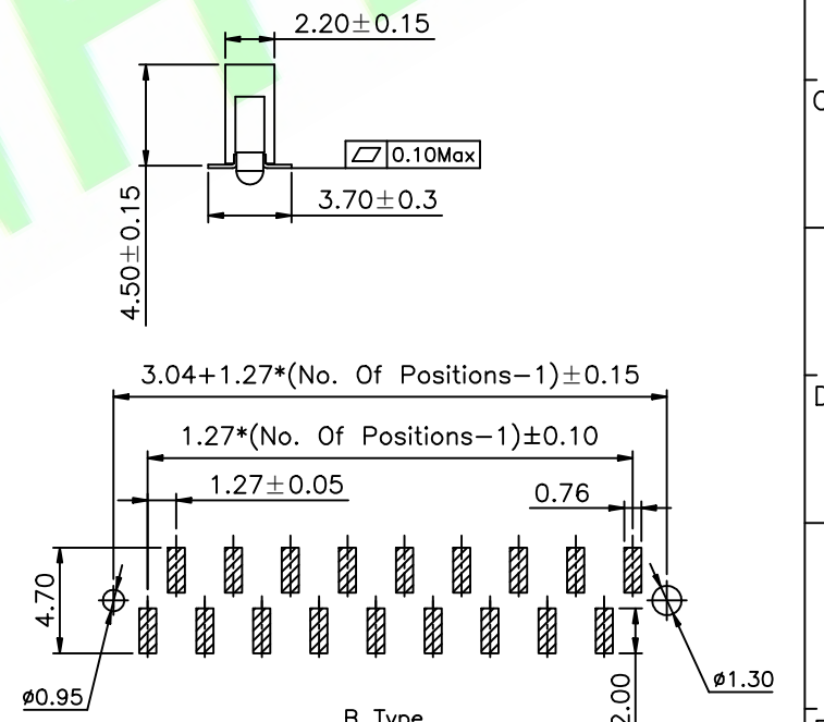
Recommended PCB Layout(Tolerance:0.05mm)
