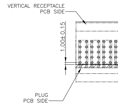
SECTION A-A (POWER CKTS ARE ALIGNED)
