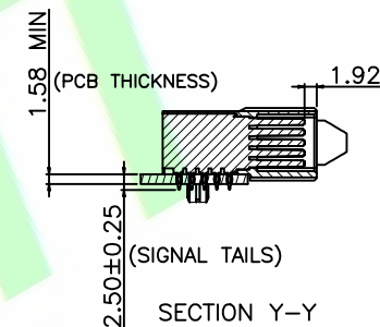
MATED PROFILE (ATED WITH VERT RECEPTACLE ASSY)
