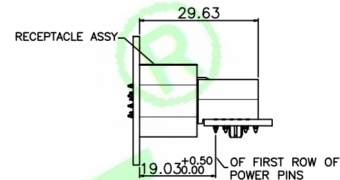
MATED PROFILE (ATED WITH VERT RECEPTACLE ASSY)
