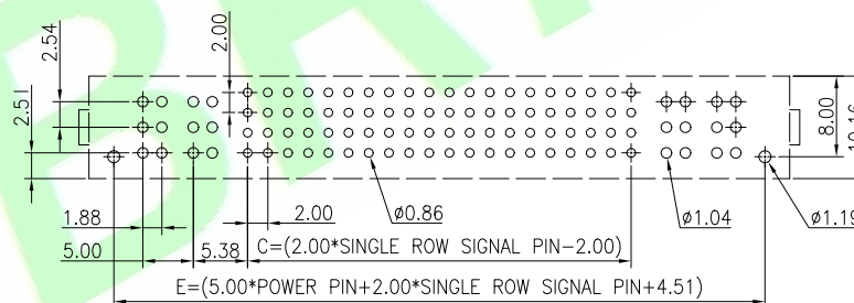
RECOMMENDED PCB LAYOUT PCB BOARD TOLERANCE ±0.05
