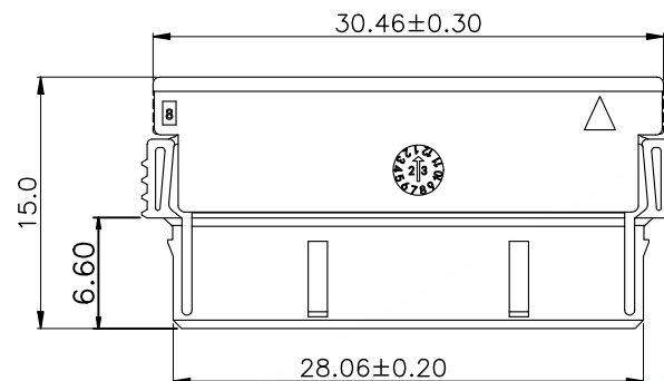
cover loose mounted
