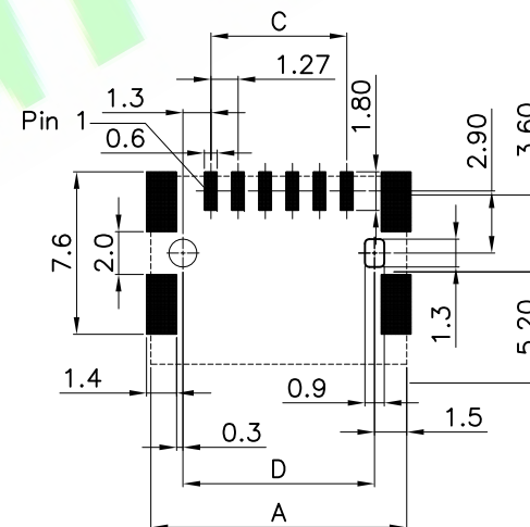
PCB Layout
