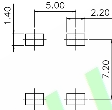
Recomended PCB Layout
