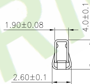
SEC C
