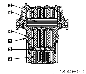
SECTION A-A WITHOUT LOCKING LEVER
