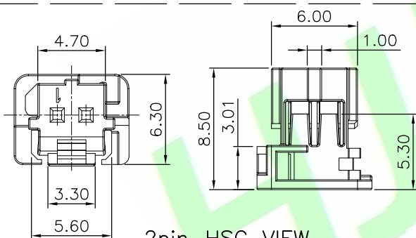
2pin_HSG VIEW
