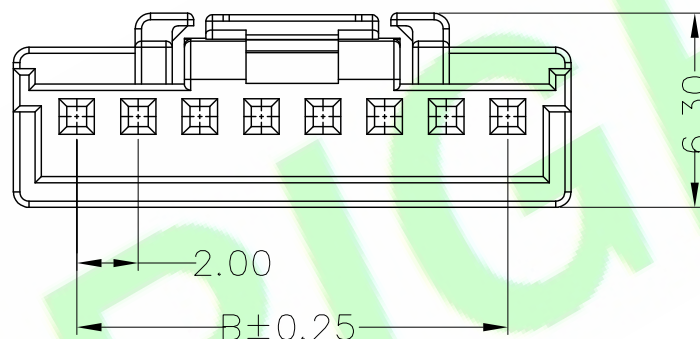
05P~15P Shape
