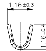
SECTION X-X
