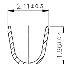
SECTION W—W
