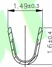
SECTION Z-Z
