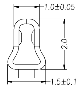
Section C-C
