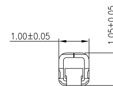
SEC:C-C
