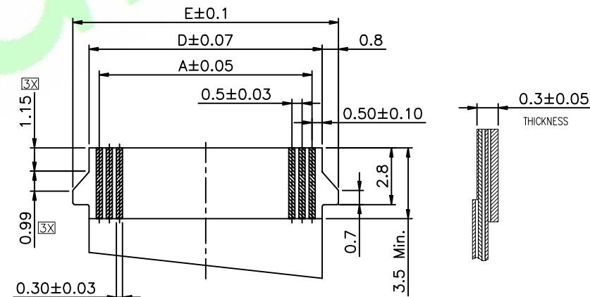
Accommodated FFC/FPC
