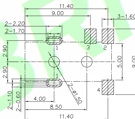
RECOMMENDED PCB LAYOUT TOP VIEW (TOLERANCE: \pm 0.05 )
