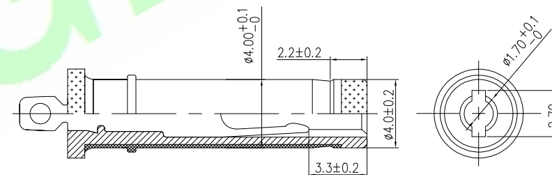
MATING PLUG P/N.: DP400170-0115-60000H
