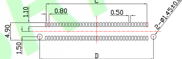
RECOMMENDED PCB LAYOUT(TOP SIDE) PCB BOARD TOLFRANCF±0.05
