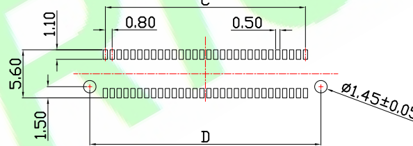
RECOMMENDED PCB LAYOUT(TOP SIDE) PCB BOARD TOLFRANCF±0.05
