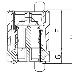
MATING HEIGHT SCALE 2:1
