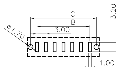
P.C. Board Hole Pattern
