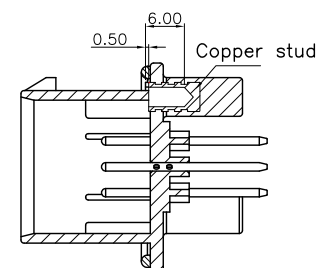
Reference drawing of embedded depth of stud
