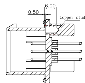
Reference drawing of embedded depth of stud
