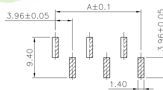
Recommended PCB Layout A Type
