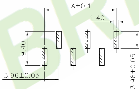
Recommended PCB Layout B Type
