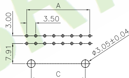
PCB Layout (4~12P)
