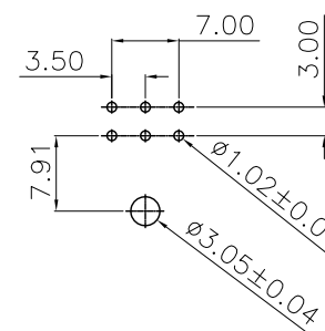
PCB Layout (2~3P)
