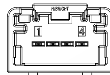
4 CIRCUIT RIGHT ANGLE HEADER POLARIZATION OPTION B TYPE COLOR:GRAY
