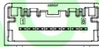
8 CIRCUIT RIGHT ANGLE HEADER POLARIZATION OPTION B TYPE COLOR:GRAY
