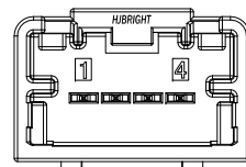
4 CIRCUIT RIGHT ANGLE HEADER POLARIZATION OPTION A TYPE COLOR:BLACK
