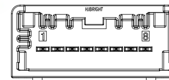
8 CIRCUIT RIGHT ANGLE HEADER POLARIZATION OPTION C TYPE COLOR:DARK GRA
