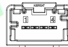
4 CIRCUIT RIGHT ANGLE HEADER POLARIZATION OPTION D TYPE COLOR:GREEN
