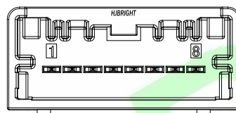
8 CIRCUIT RIGHT ANGLE HEADER POLARIZATION OPTION A TYPE COLOR:BLACK
