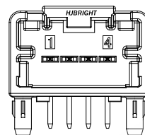
4 CIRCUIT RIGHT ANGLE HEADER POLARIZATION OPTION A
