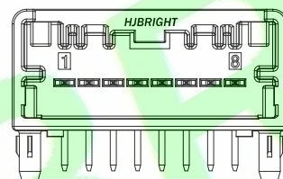
8 CIRCUIT RIGHT ANGLE HEADER POLARIZATION OPTION A
