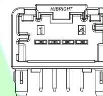
4 CIRCUIT RIGHT ANGLE HEADER POLARIZATION OPTION D
