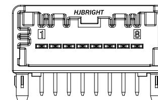
8 CIRCUIT RIGHT ANGLE HEADER POLARIZATION OPTION C
