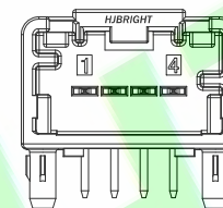
4 CIRCUIT RIGHT ANGLE HEADER POLARIZATION OPTION C
