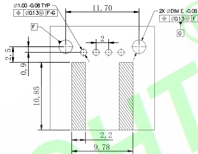
PCB LAYOUT
