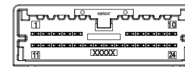
24 CIRCUIT RIGHT ANGLE HEADER POLARIZATION OPTION C TYPE COLOR:DARK GRAY
