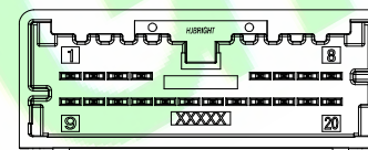
20 CIRCUIT RIGHT ANGLE HEADER POLARIZATION OPTION B TYPE COLOR:GRAY
