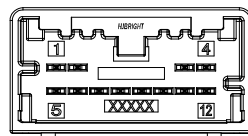
12 CIRCUIT RIGHT ANGLE HEADER POLARIZATION OPTION A TYPE COLOR:BLACK
