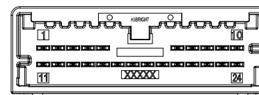
24 CIRCUIT RIGHT ANGLE HEADER POLARIZATION OPTION B TYPE COLOR:GRAY
