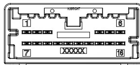
16 CIRCUIT RIGHT ANGLE HEADER POLARIZATION OPTION A TYPE COLOR:DARK BLACK
