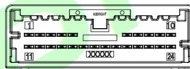
24 CIRCUIT RIGHT ANGLE HEADER POLARIZATION OPTION A TYPE COLOR:DARK BLACK
