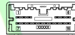
16 CIRCUIT RIGHT ANGLE HEADER POLARIZATION OPTION C TYPE COLOR:DARK GRAY
