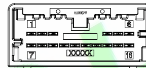
16 CIRCUIT RIGHT ANGLE HEADER POLARIZATION OPTION B TYPE COLOR:GRAY
