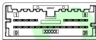
20 CIRCUIT RIGHT ANGLE HEADER POLARIZATION OPTION A TYPE COLOR:DARK BLACK
