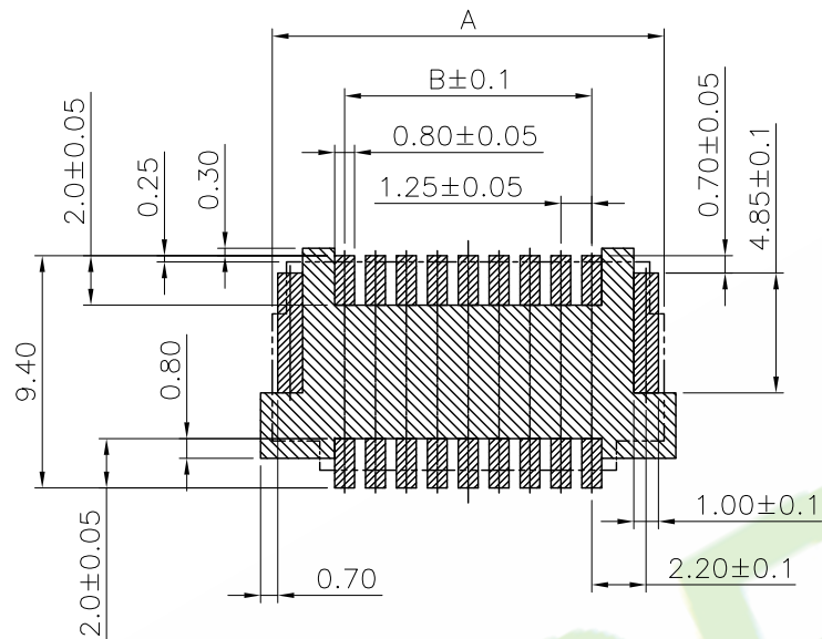
PCB LAYOUT
