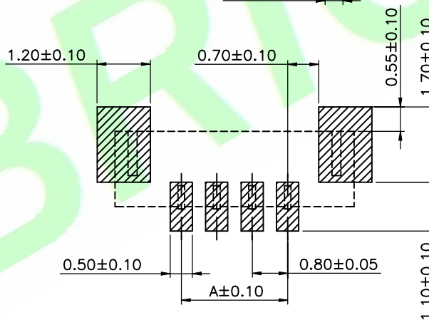
PCB LAYOUT
