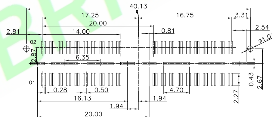
Recommended PCB Layout unmarked tolerance:±0.05
