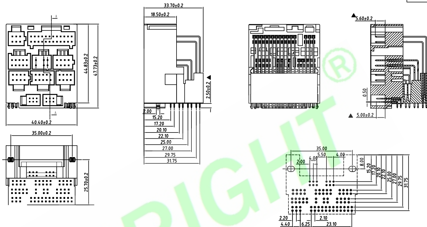
Dimensions of PC board holes (Tolerance : \pm 0.1 )
