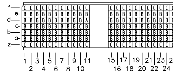
Contact Layout
