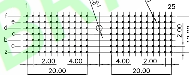
Recommended PCB Layout (Tolerance:0.05mm)
