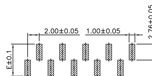
B Type
