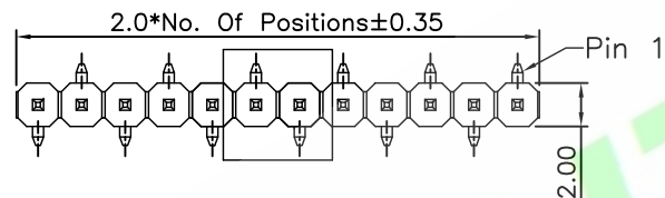
B Type
