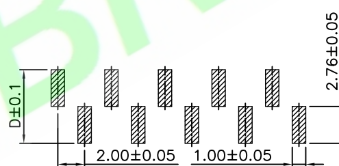
A Type
