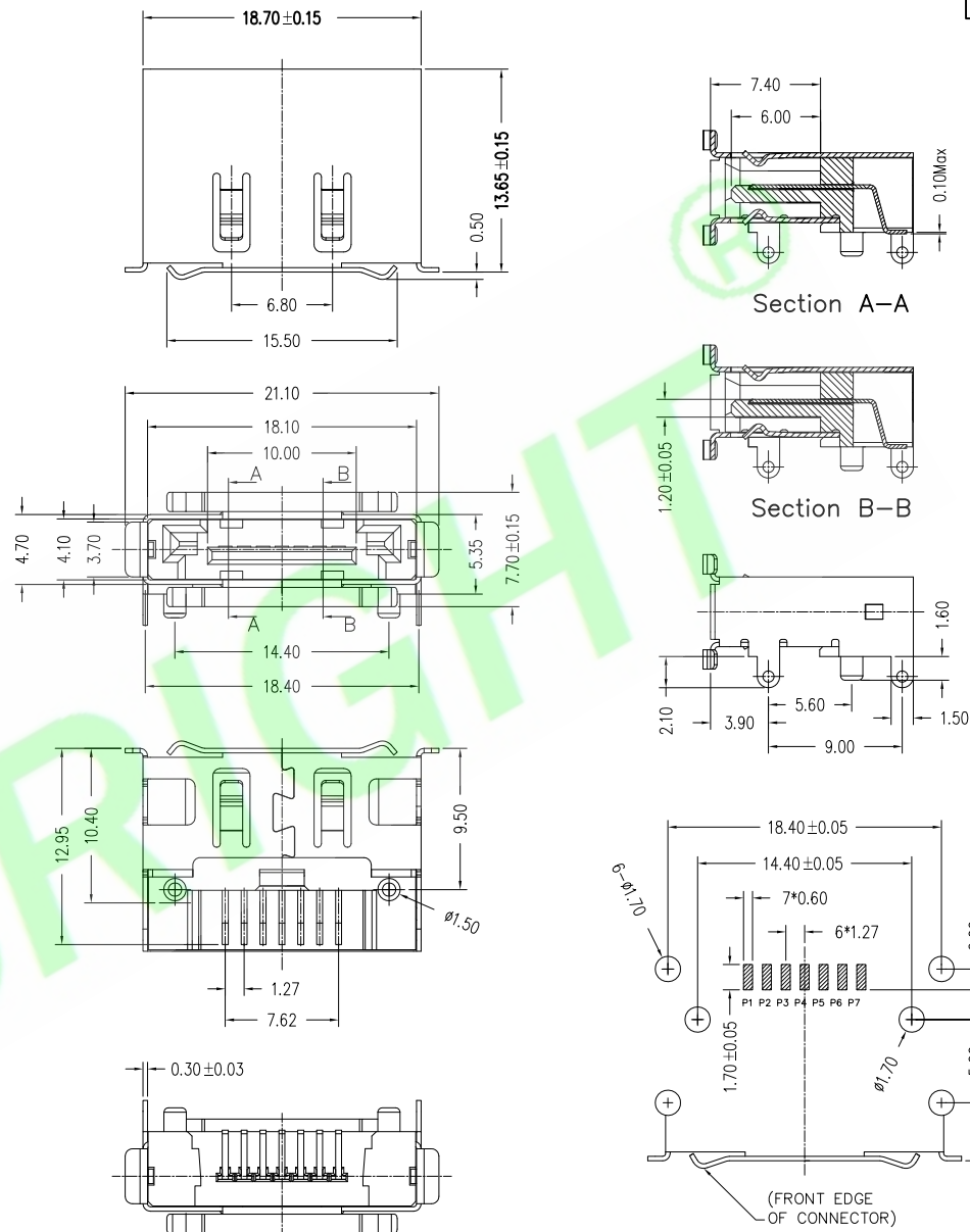
Recommended PCB Layout
