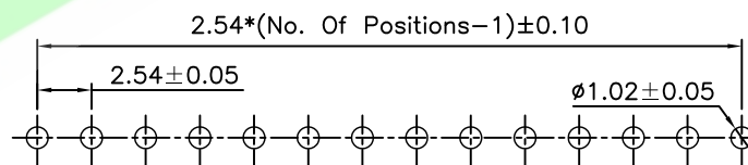
Recommended PCB Layout
